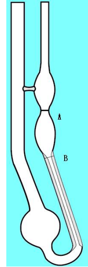
Fig.6 Cannon-Fenske Viscometer.
